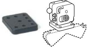
OFFSET BRACKET Allows axial displacement between measuring units to be able to rotate past projecting machine parts.
