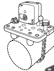
SLIDING FIXTURE Used when the shafts cannot be rotated. Part Nr: 12-0039
